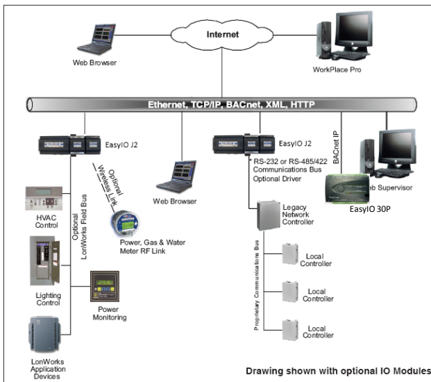
Drawing shown with optional IO Modules
